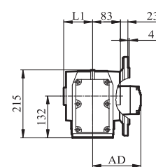
GKAF/GKHF/GKVF57
