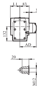
GKA/GKH/GKV57
