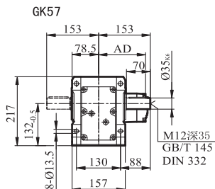
GKA/GKH/GKV57
