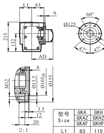
GKAF/GKHF/GKVF57
