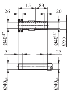
GKH/GKHZ/GKHF57输出轴
