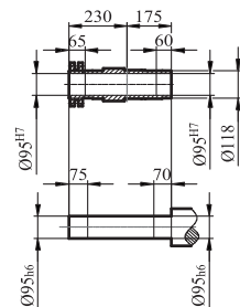
GKH/GKHZ/GKHF107输出轴
