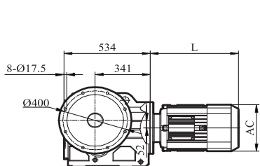
GKA107T
