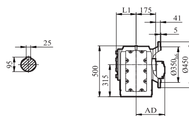
GKAF/GKHF/GKVF107
