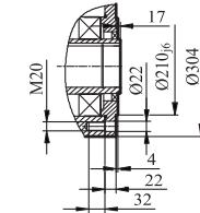
GKAF/GKHF/GKVF107
