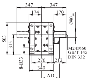
GKA/GKH/GKV107
