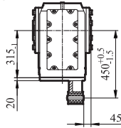
GKH/GKHZ/GKHF107输出轴
